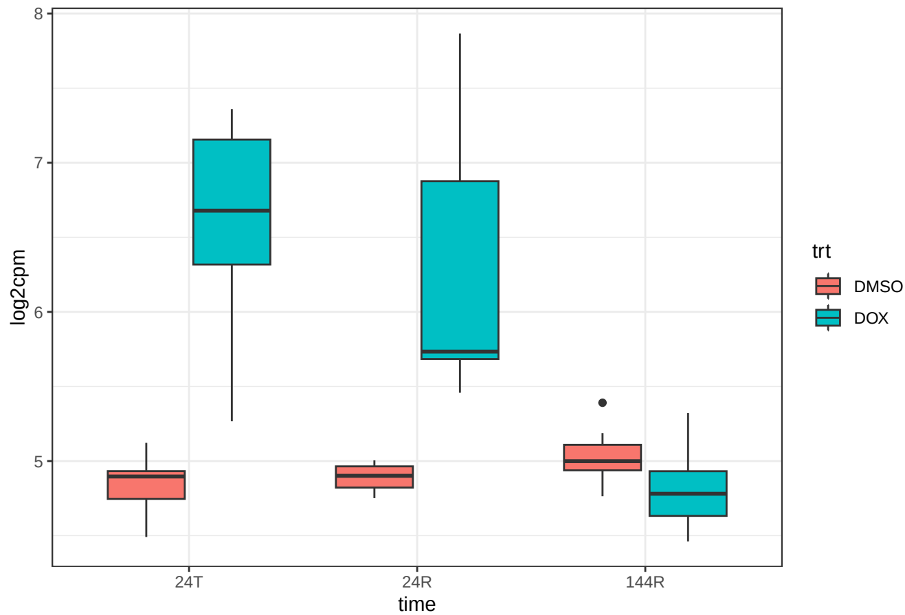
gene 374383 NCR3LG1 dist 0
